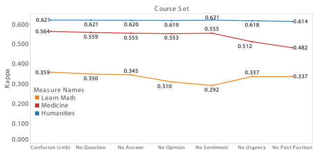
Figure 3: Ablative Analysis, Kappas. Minus question is the combined classifier without the question constituent; minus answer is minus question without the answer constituent; and so on.
