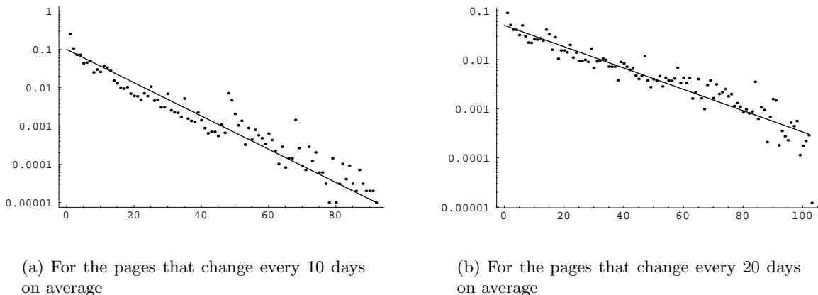
Figure 6: Change intervals of pages
