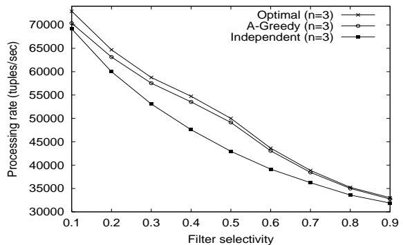
Figure 10: Effect of selectivity under convergence
