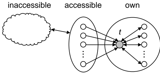
Figure 2: An optimal link structure for PageRank.
