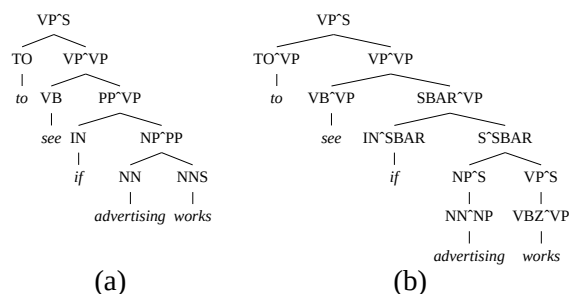
Figure 5: An error resolved with the TAG-PA annotation (of the IN tag): (a) the incorrect baseline parse and (b) the correct TAG-PA parse. SPLIT-IN also resolves this error.
